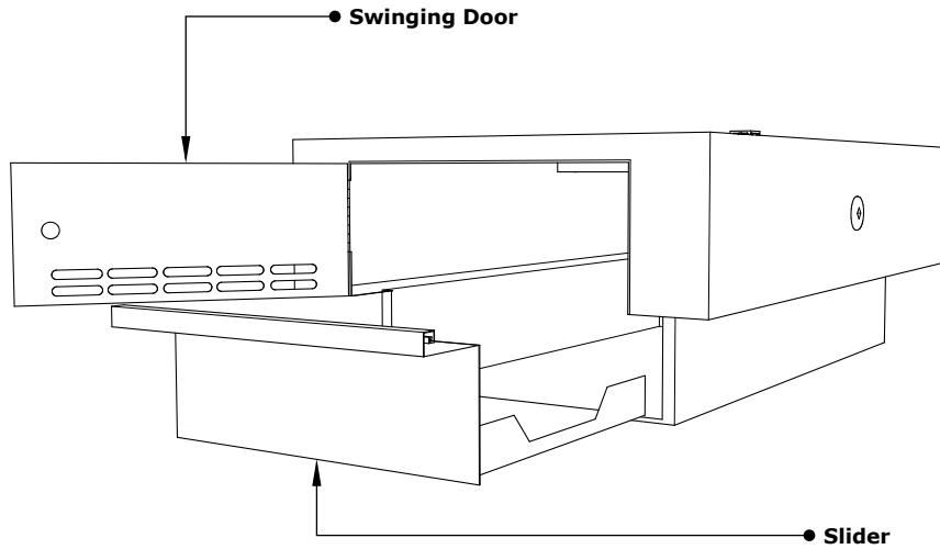
ISOMETRIC VIEW
