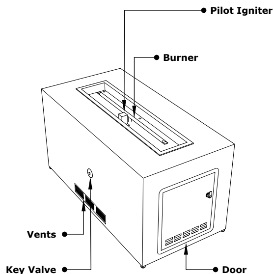
ISOMETRIC VIEW
