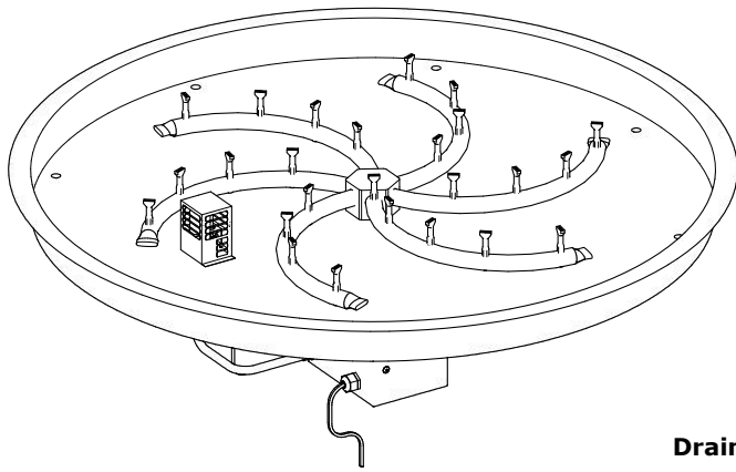
ISOMETRIC VIEW
